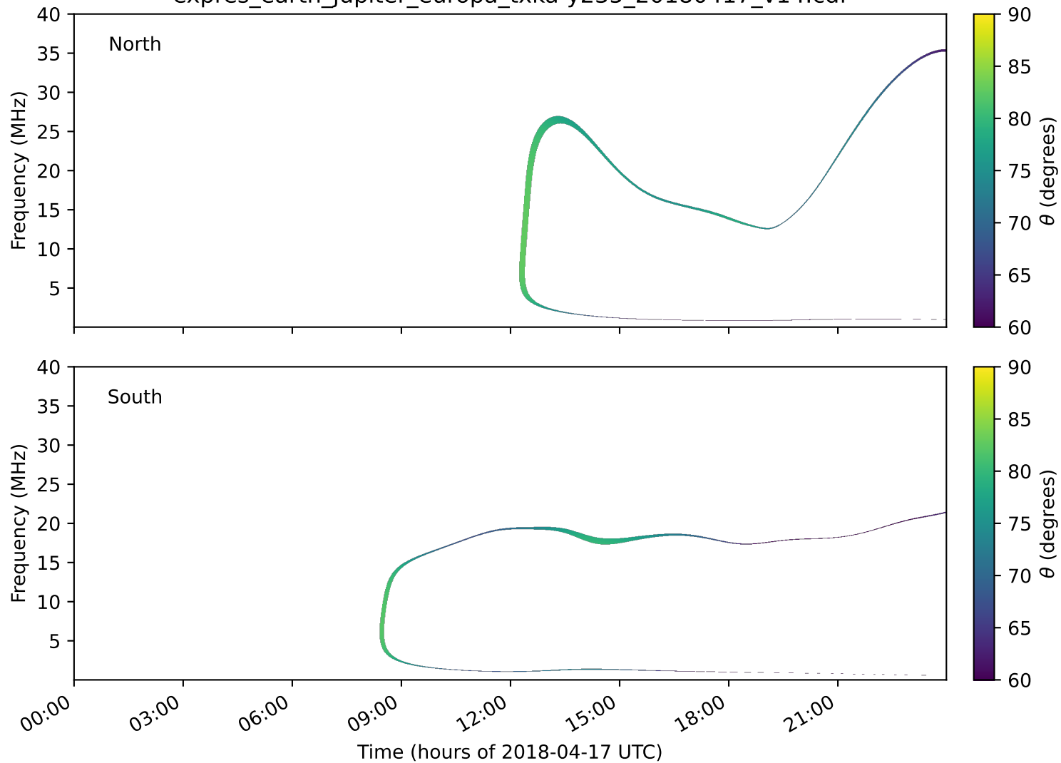
expres_earth_jupiter_europa_txka-y235_20180417_v14.cdf
