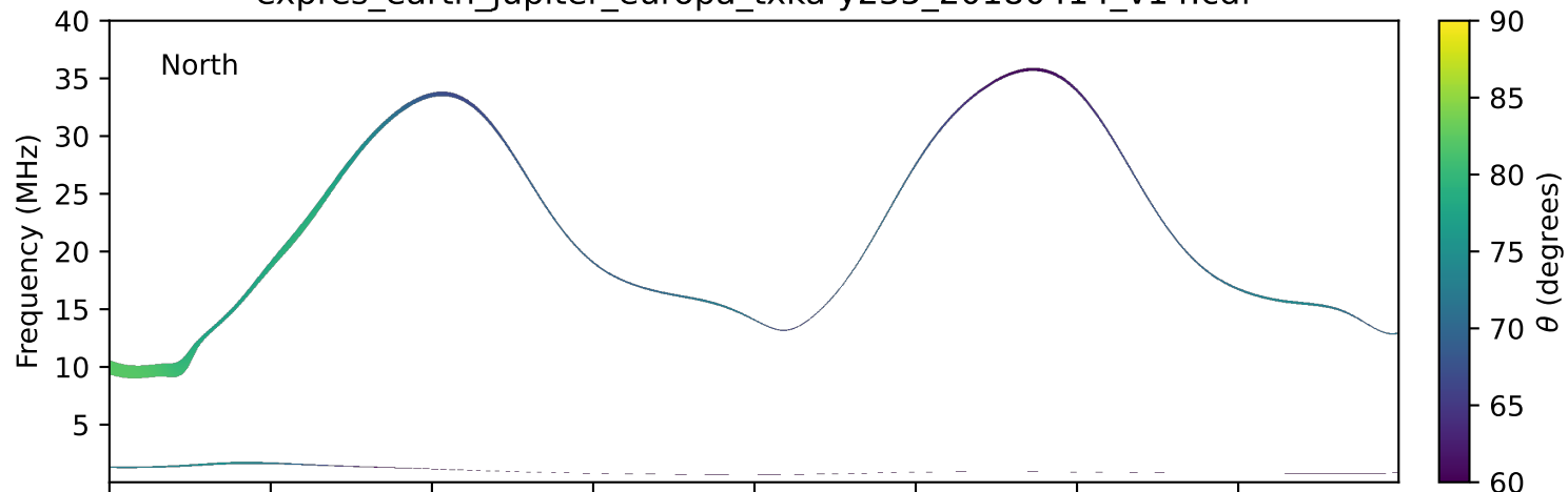
expres_earth_jupiter_europa_txka-y235_20180414_v14.cdf
