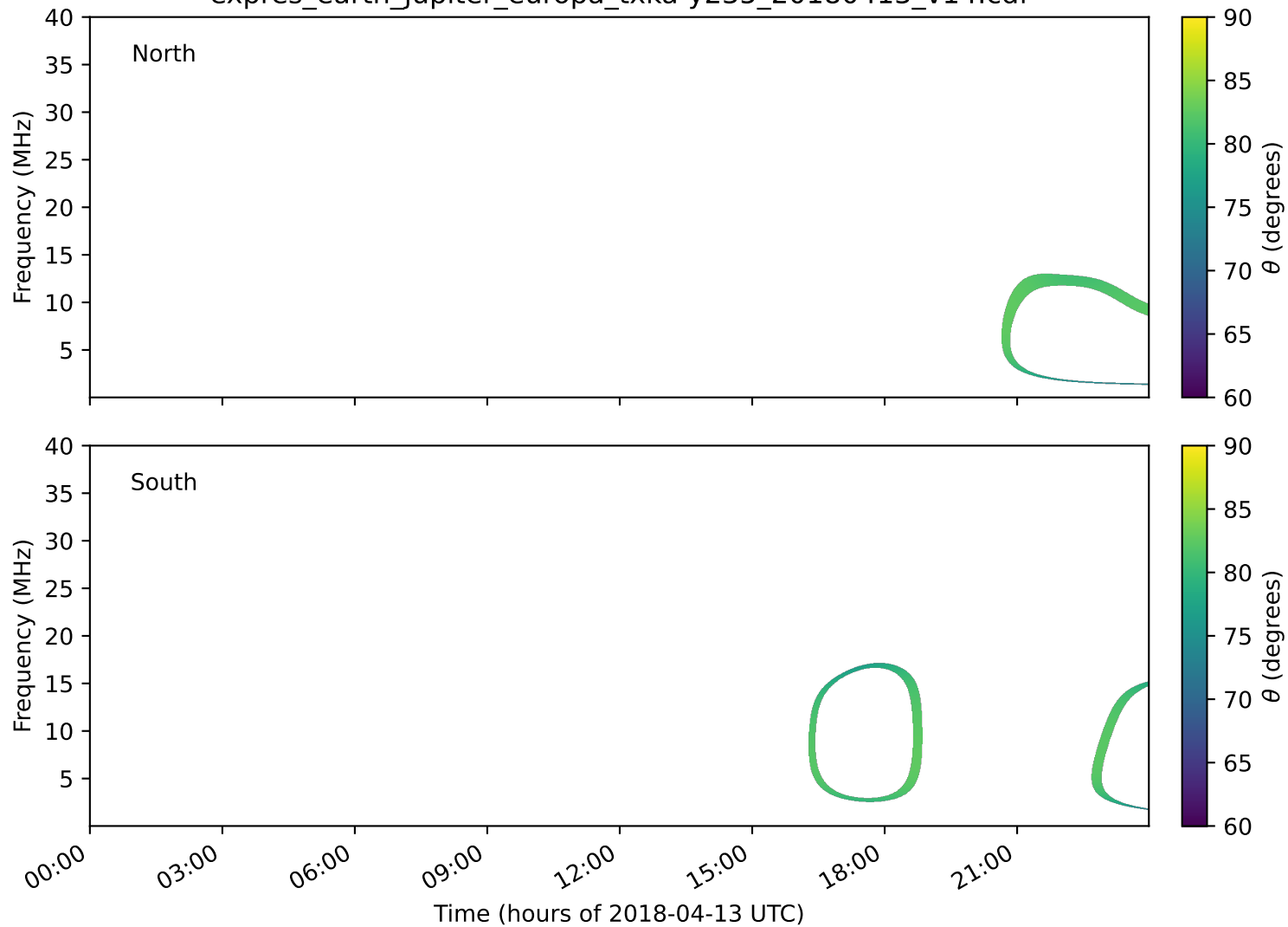
expres_earth_jupiter_europa_txka-y235_20180413_v14.cdf
