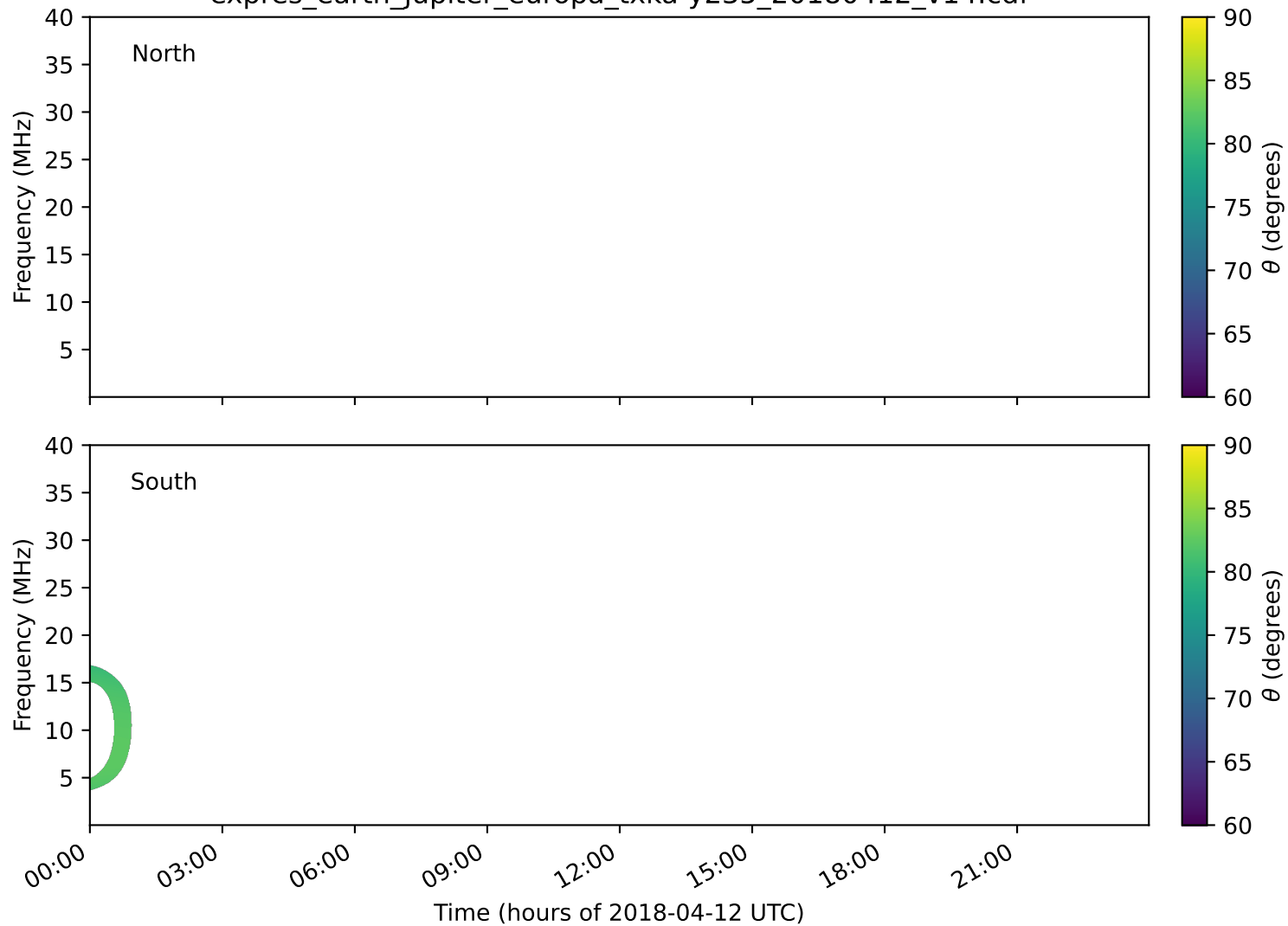
expres_earth_jupiter_europa_txka-y235_20180412_v14.cdf
