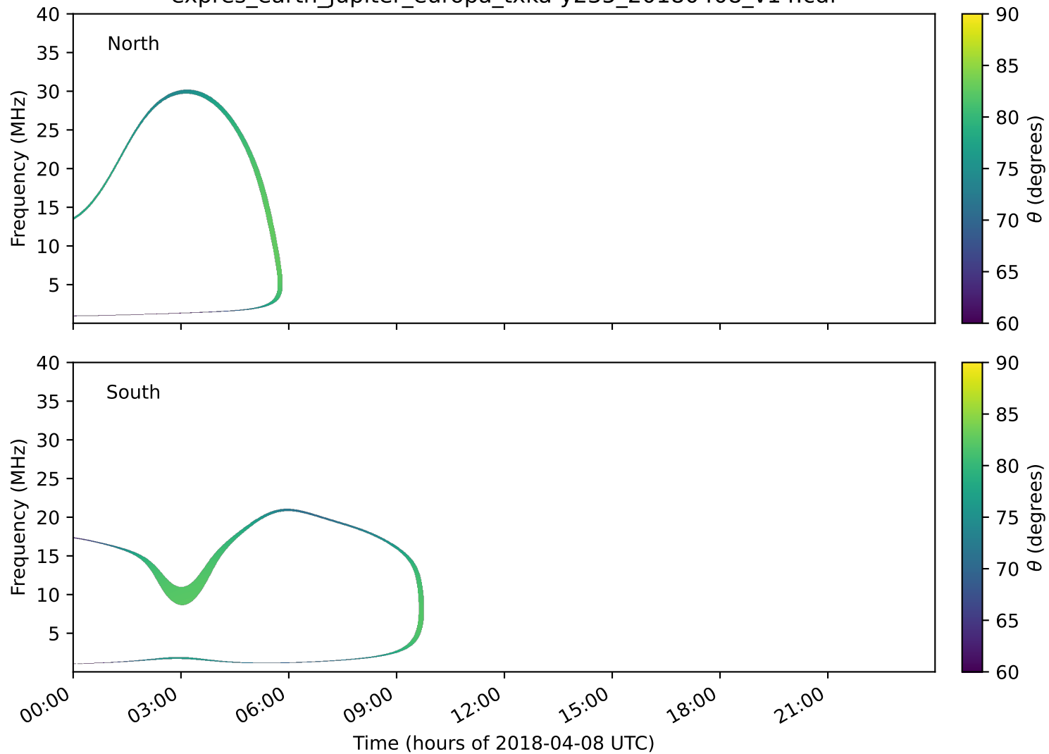
expres_earth_jupiter_europa_txka-y235_20180408_v14.cdf
