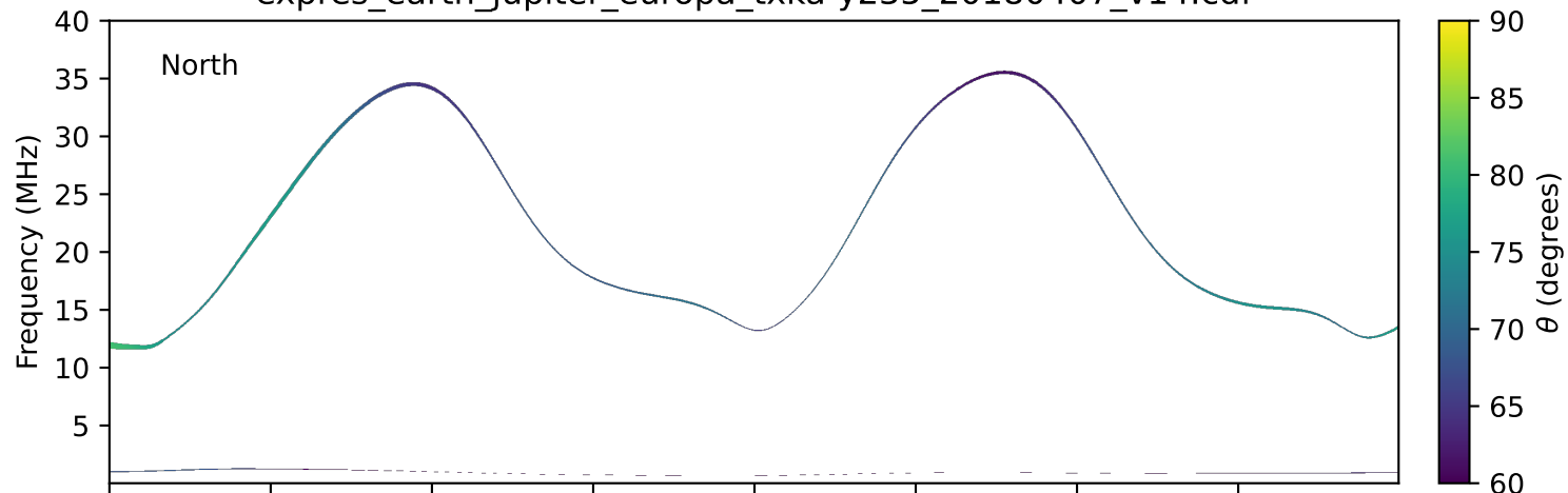
expres_earth_jupiter_europa_txka-y235_20180407_v14.cdf
