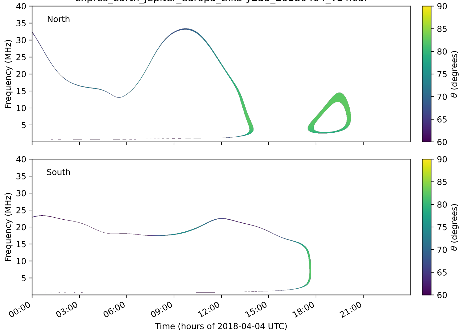
expres_earth_jupiter_europa_txka-y235_20180404_v14.cdf
