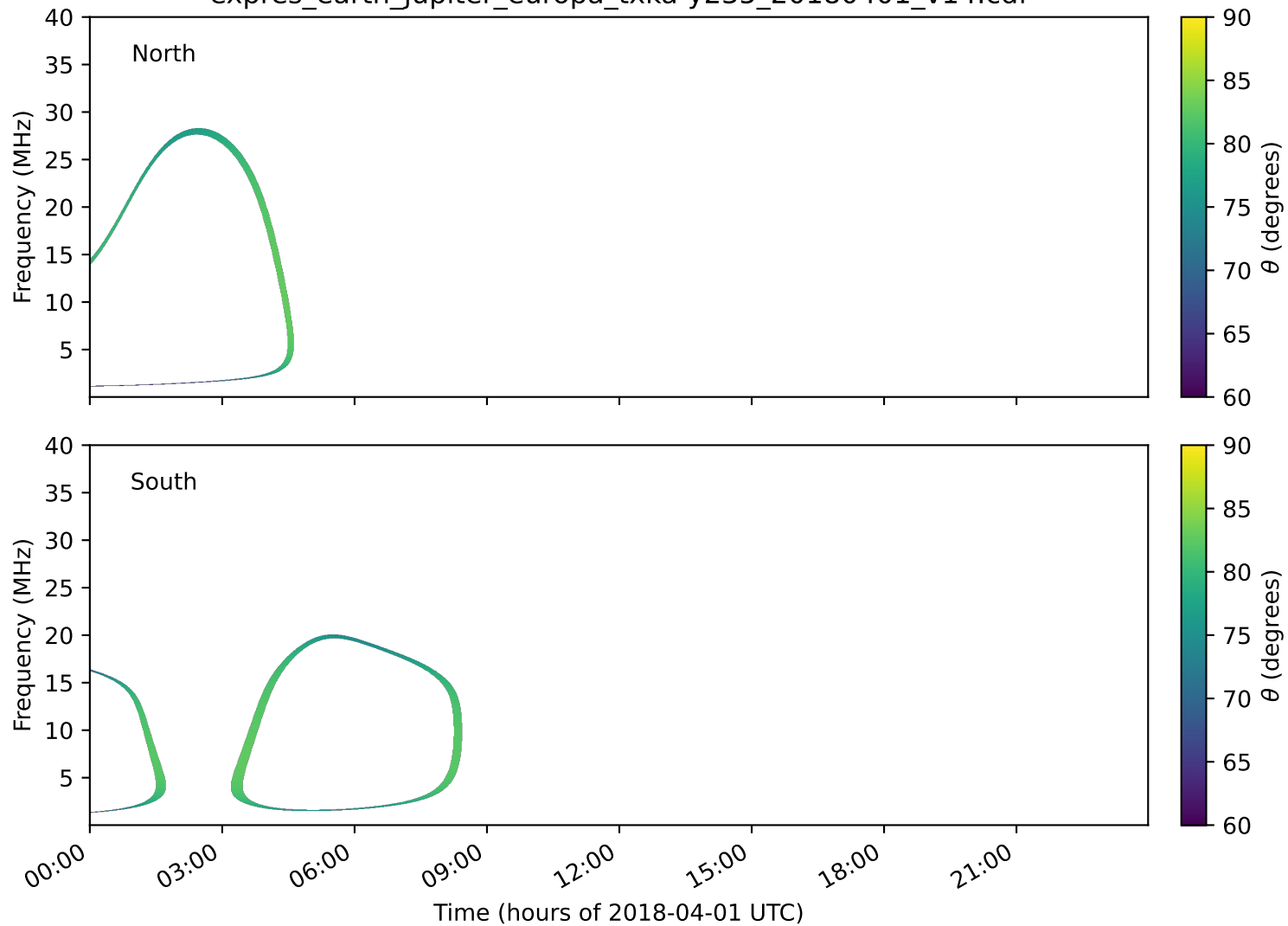
expres_earth_jupiter_europa_txka-y235_20180401_v14.cdf
