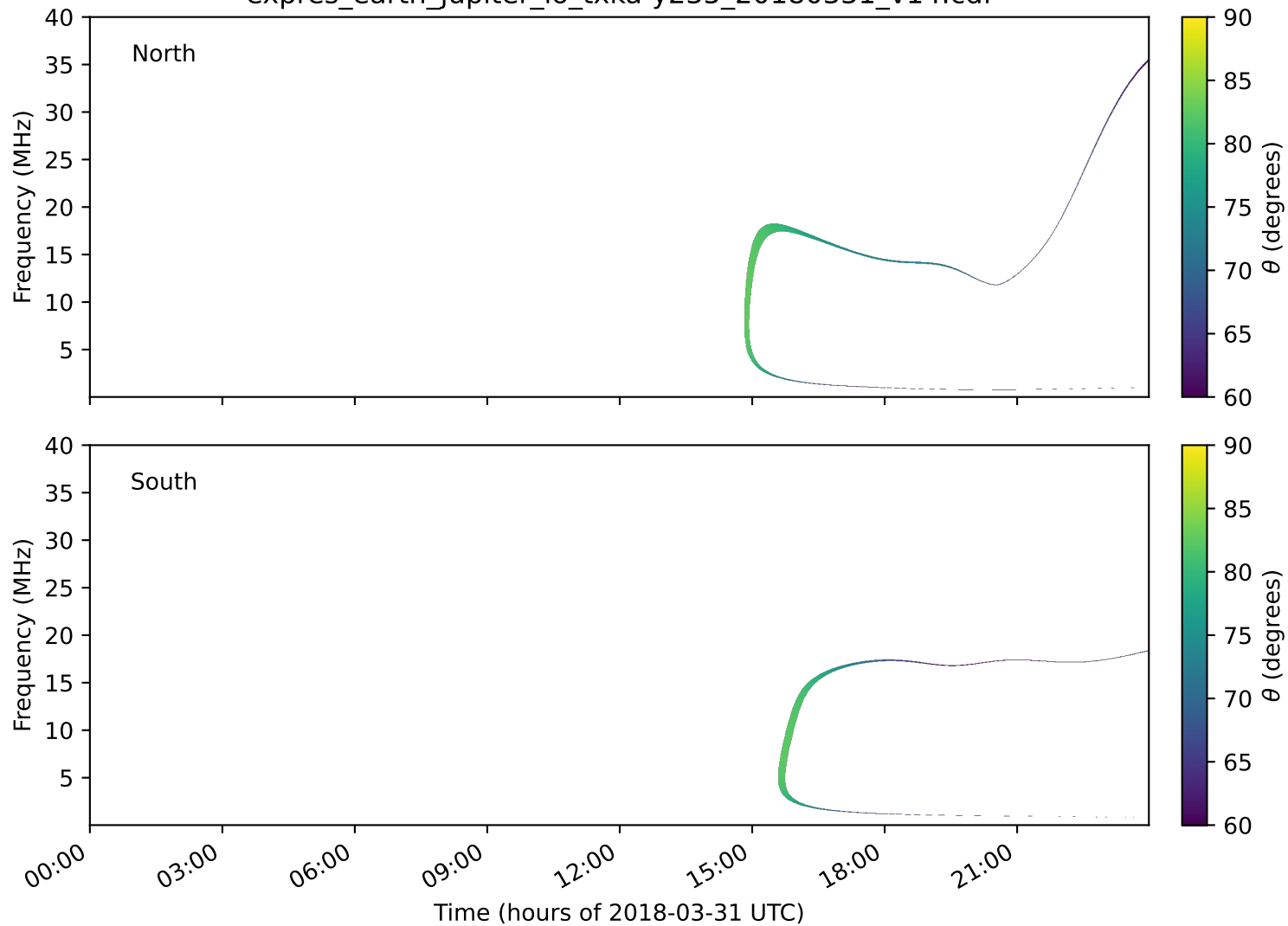
expres_earth_jupiter_io_txka-y235_20180331_v14.cdf
