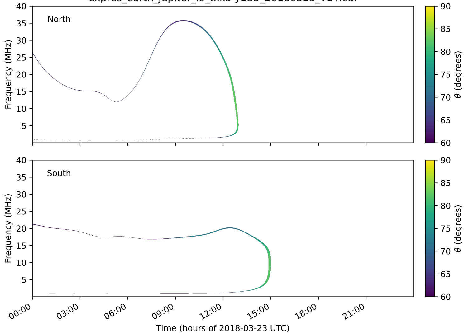
expres_earth_jupiter_io_txka-y235_20180323_v14.cdf
