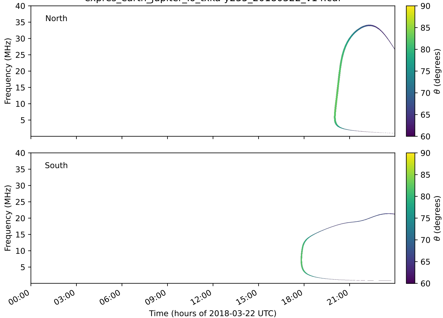
expres_earth_jupiter_io_txka-y235_20180322_v14.cdf
