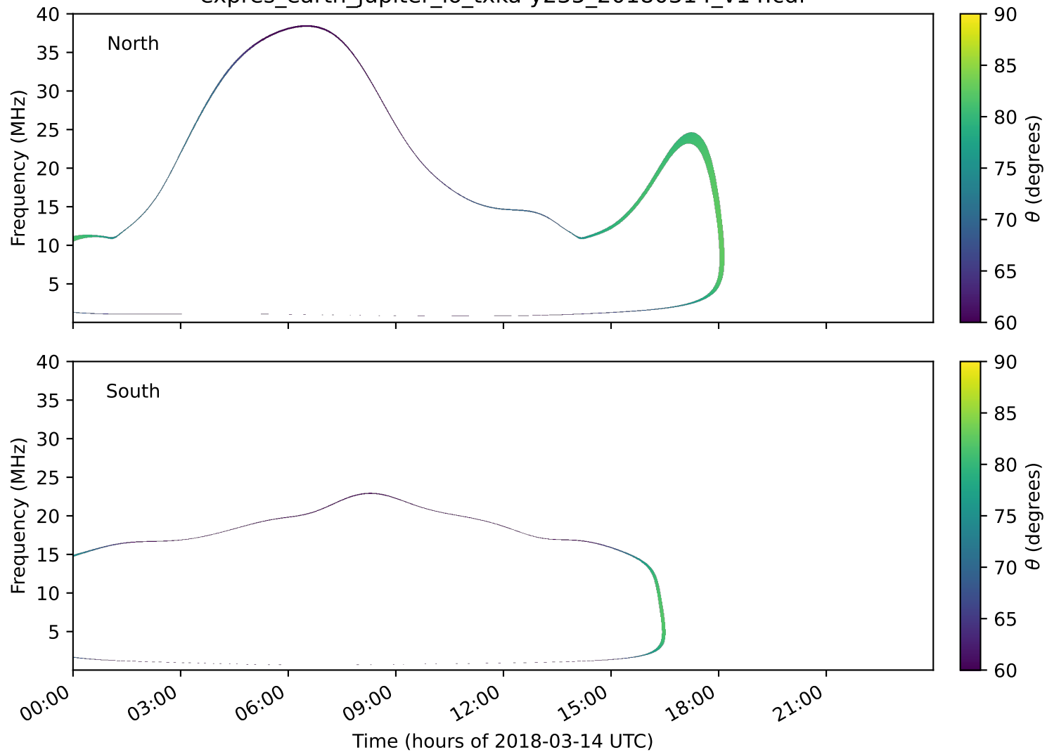
expres_earth_jupiter_io_txka-y235_20180314_v14.cdf
