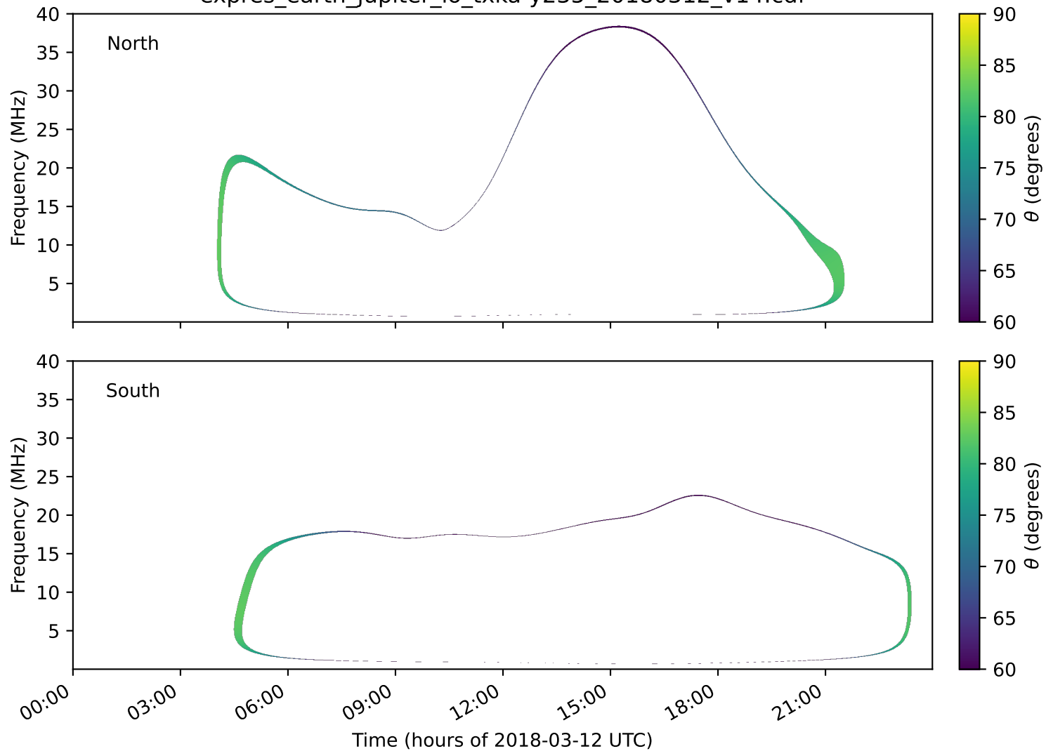
expres_earth_jupiter_io_txka-y235_20180312_v14.cdf
