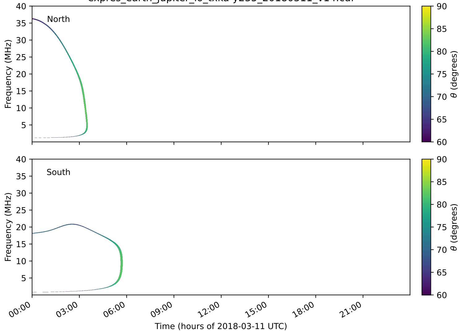
expres_earth_jupiter_io_txka-y235_20180311_v14.cdf
