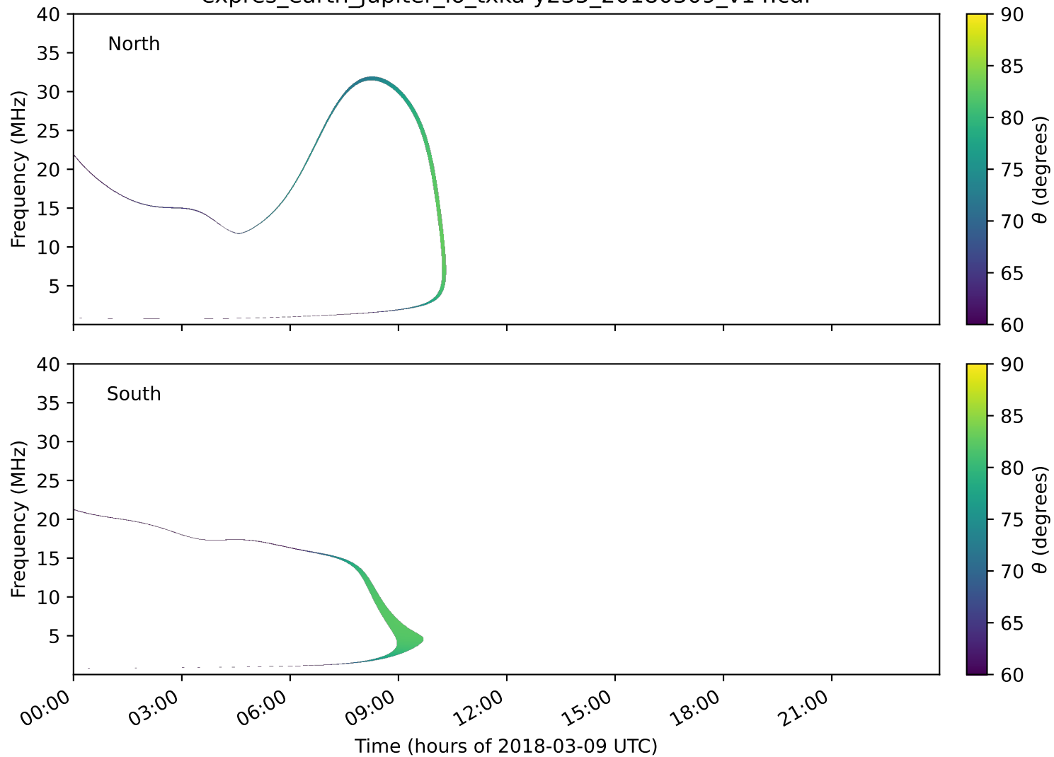
expres_earth_jupiter_io_txka-y235_20180309_v14.cdf
