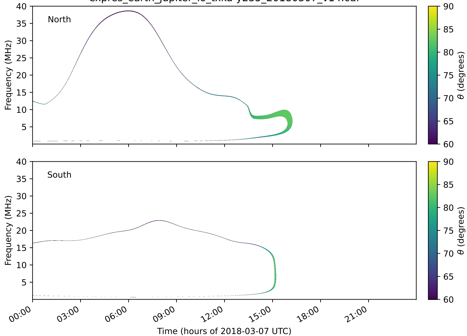
expres_earth_jupiter_io_txka-y235_20180307_v14.cdf
