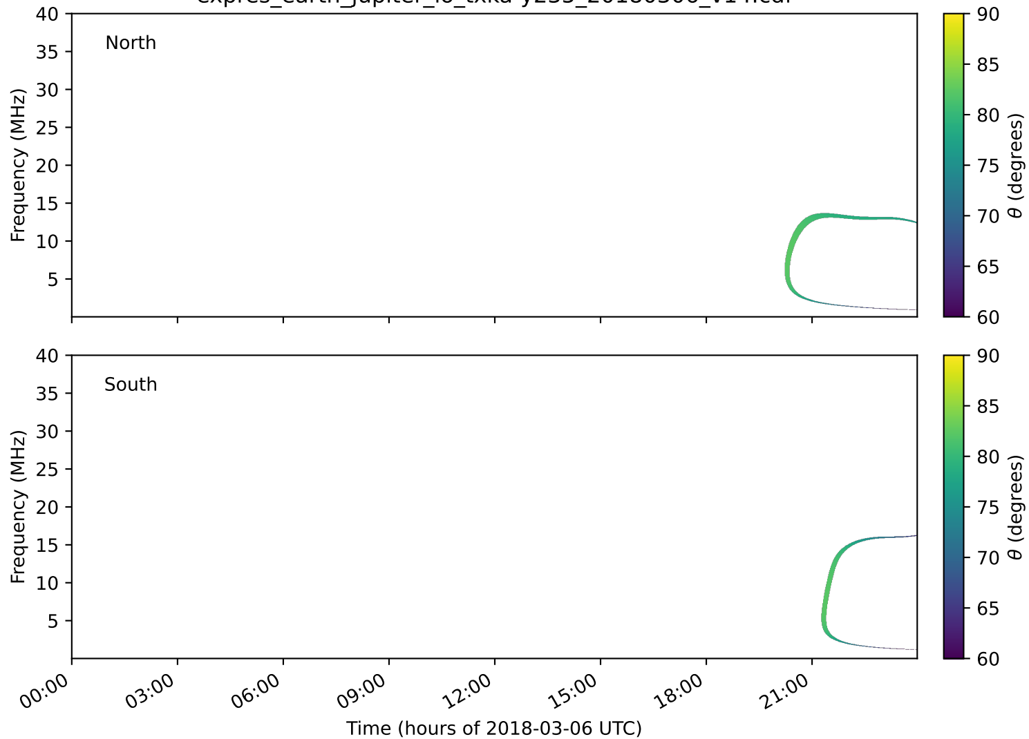
expres_earth_jupiter_io_txka-y235_20180306_v14.cdf
