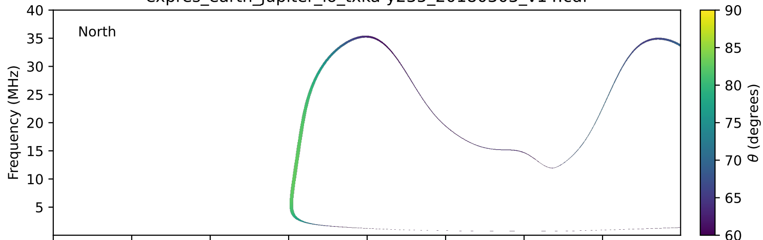
expres_earth_jupiter_io_txka-y235_20180303_v14.cdf
