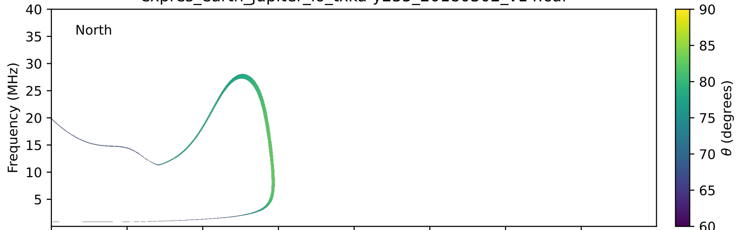
expres_earth_jupiter_io_txka-y235_20180302_v14.cdf
