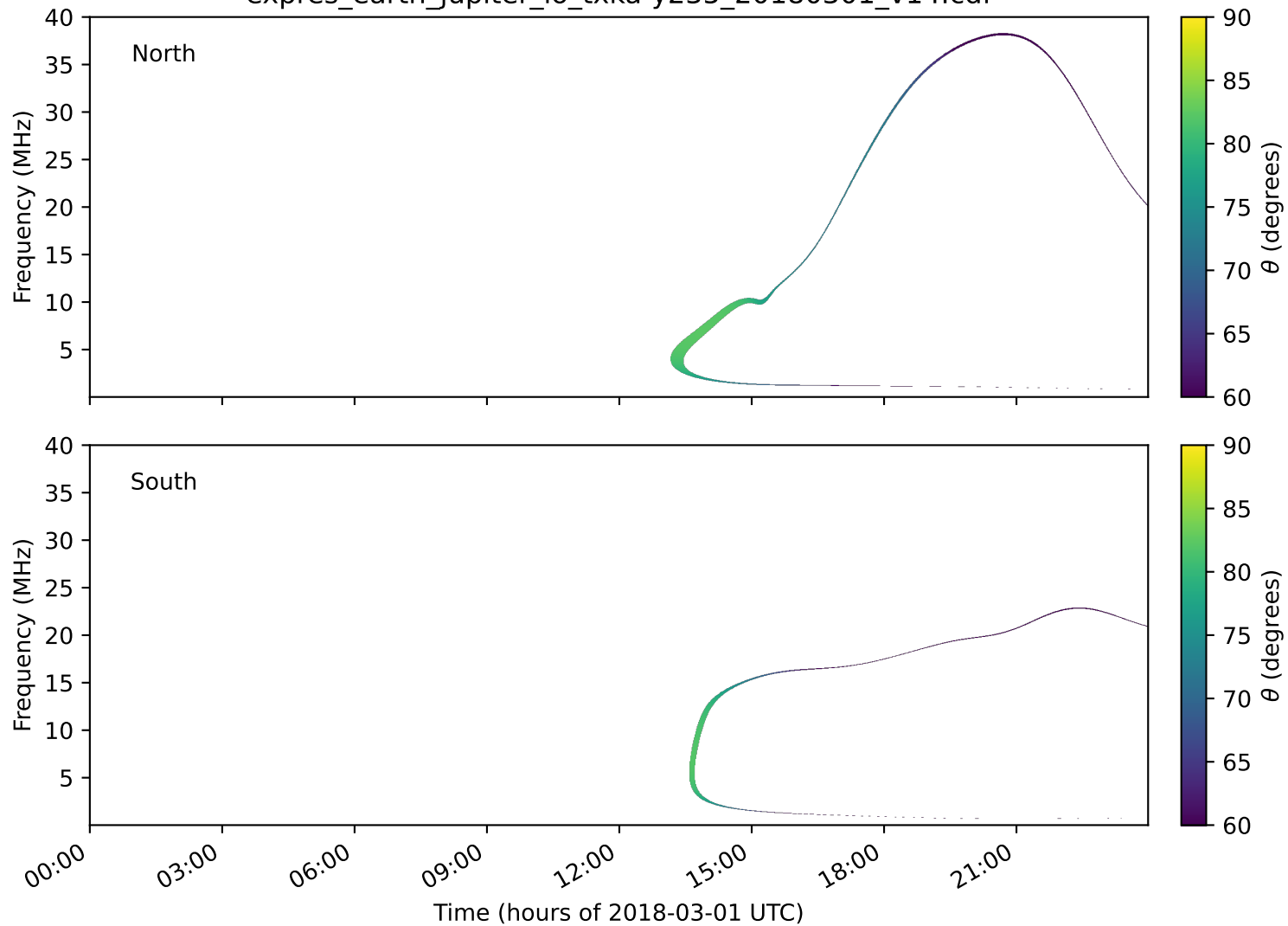
expres_earth_jupiter_io_txka-y235_20180301_v14.cdf
