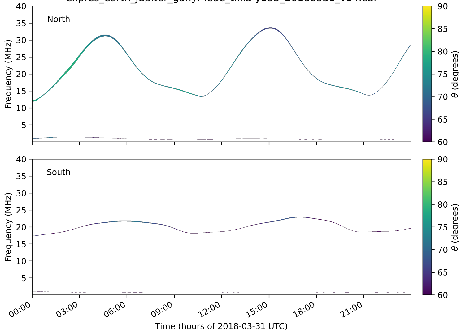
expres_earth_jupiter_ganymede_txka-y235_20180331_v14.cdf
