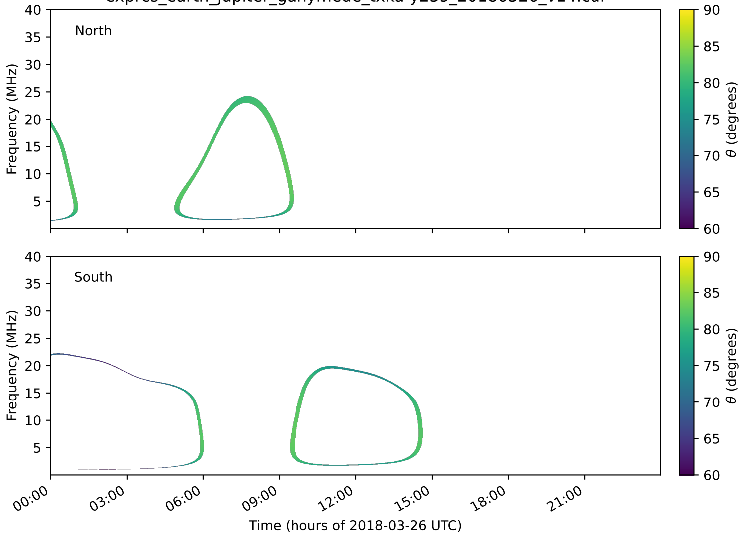
expres_earth_jupiter_ganymede_txka-y235_20180326_v14.cdf
