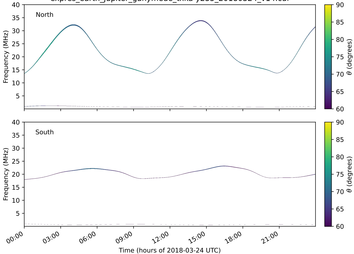
expres_earth_jupiter_ganymede_txka-y235_20180324_v14.cdf
