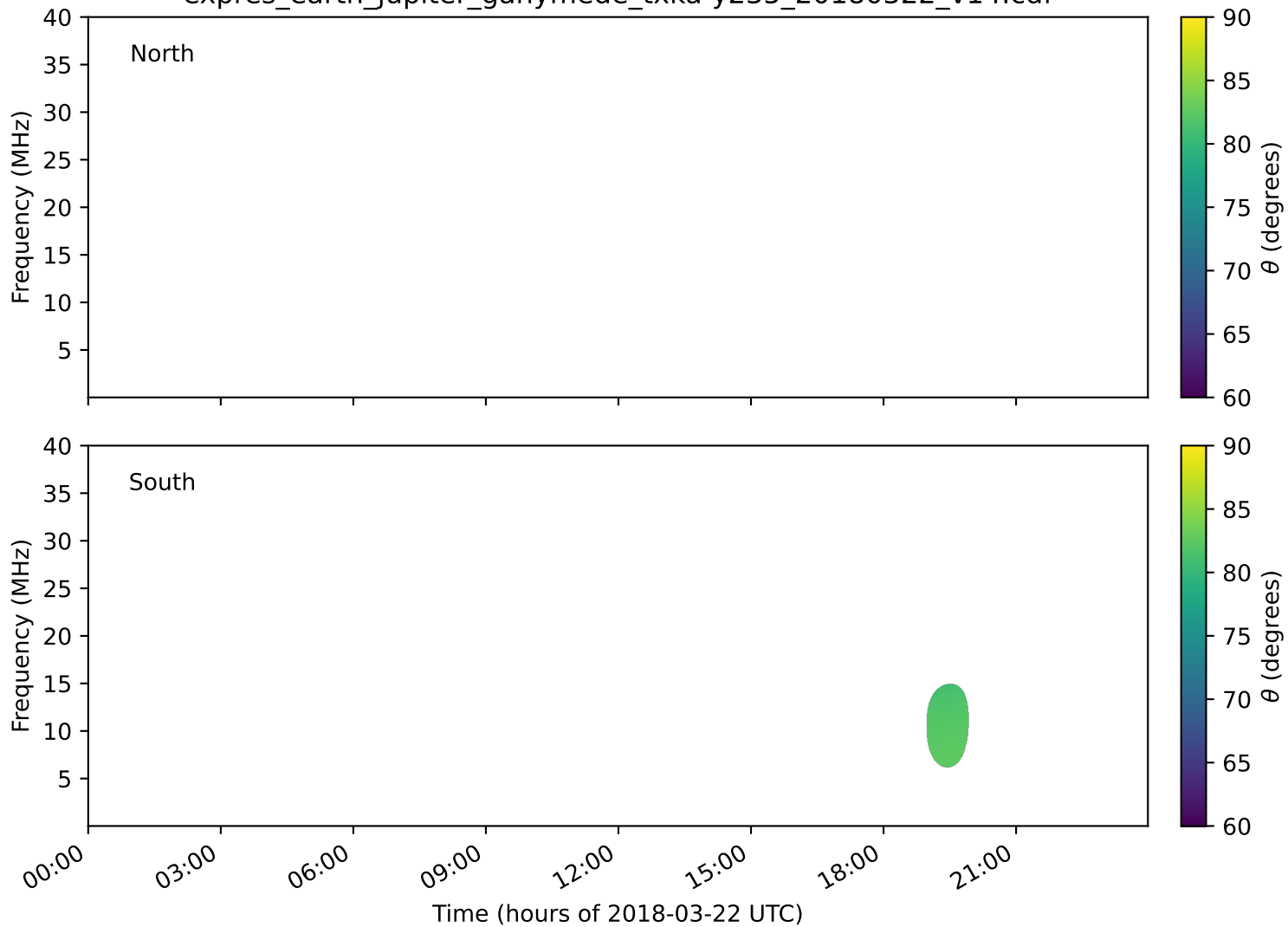
expres_earth_jupiter_ganymede_txka-y235_20180322_v14.cdf
