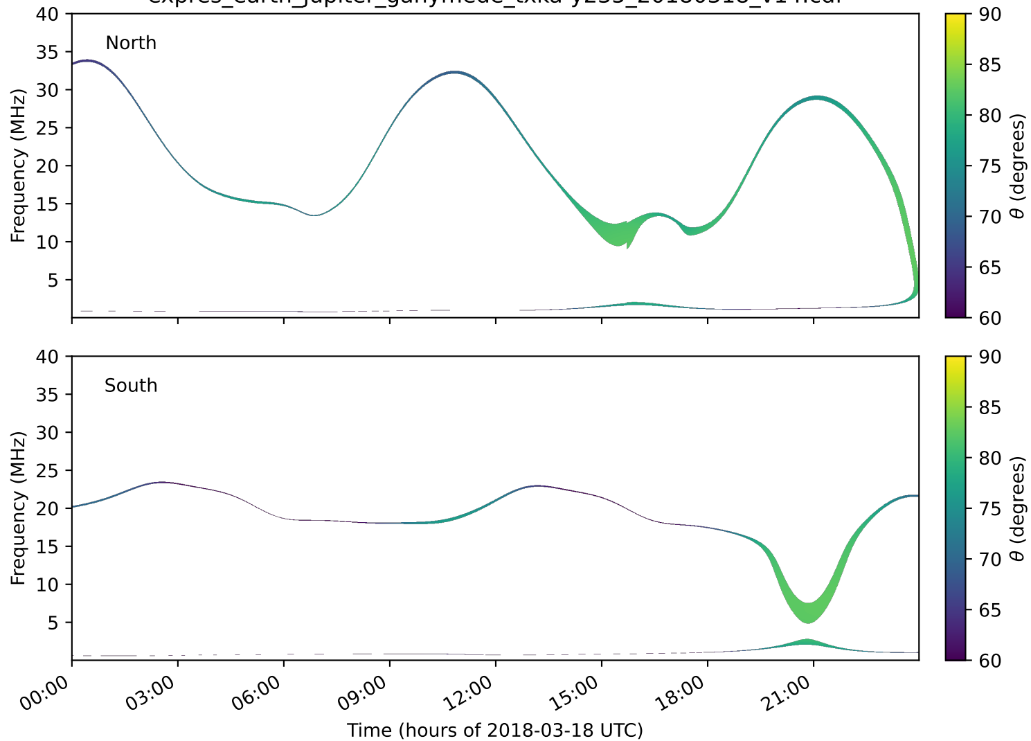
expres_earth_jupiter_ganymede_txka-y235_20180318_v14.cdf
