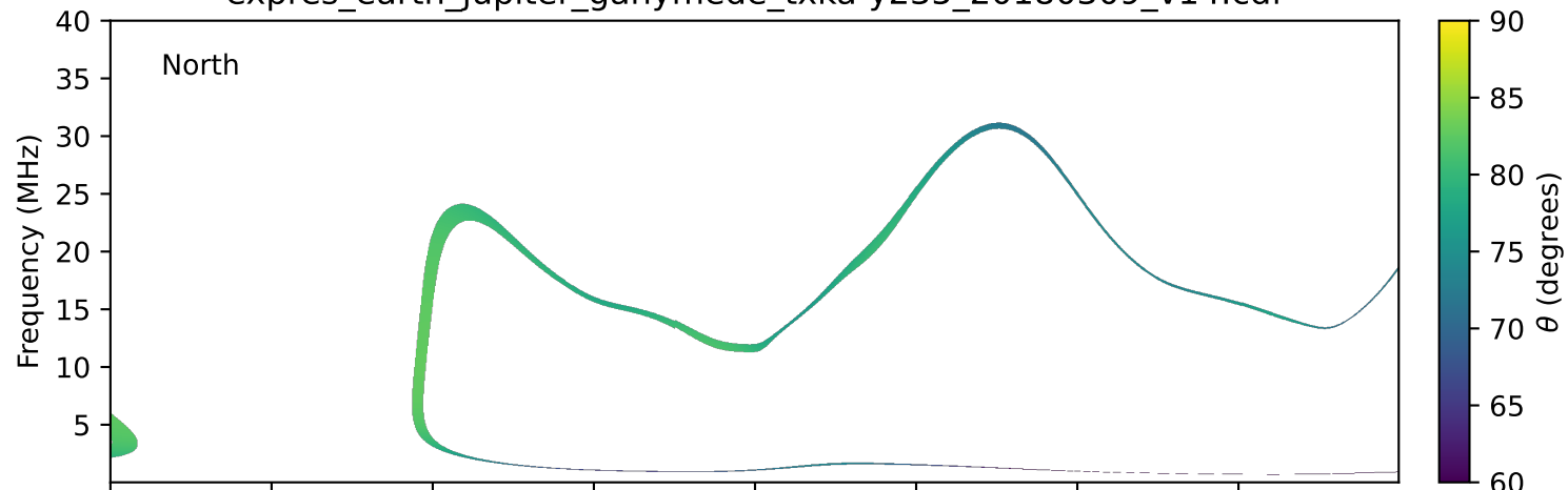
expres_earth_jupiter_ganymede_txka-y235_20180309_v14.cdf
