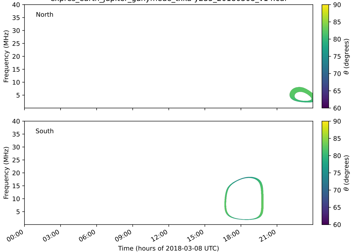
expres_earth_jupiter_ganymede_txka-y235_20180308_v14.cdf
