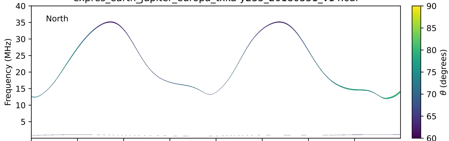
expres_earth_jupiter_europa_txka-y235_20180331_v14.cdf
