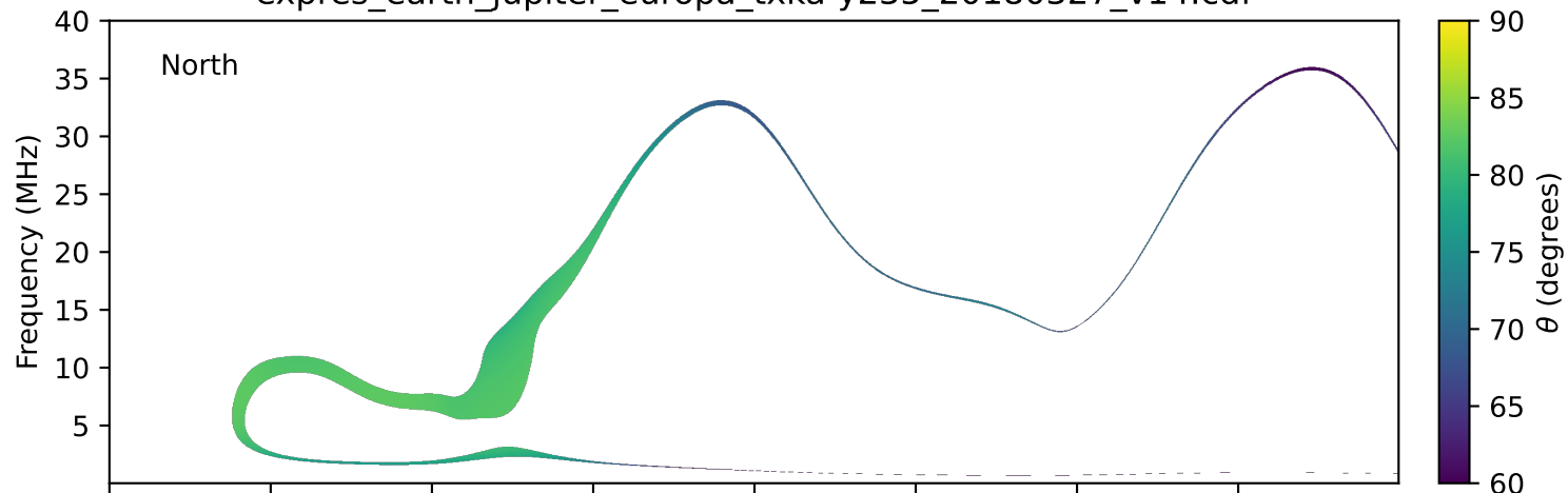
expres_earth_jupiter_europa_txka-y235_20180327_v14.cdf
