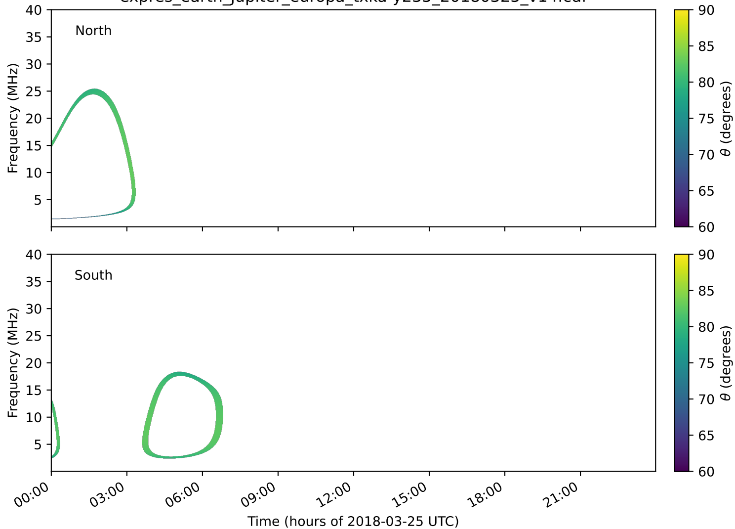
expres_earth_jupiter_europa_txka-y235_20180325_v14.cdf
