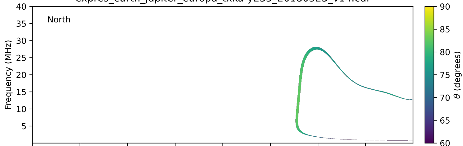
expres_earth_jupiter_europa_txka-y235_20180323_v14.cdf
