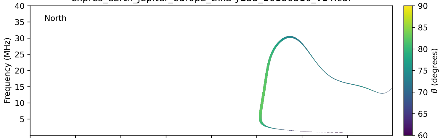
expres_earth_jupiter_europa_txka-y235_20180316_v14.cdf
