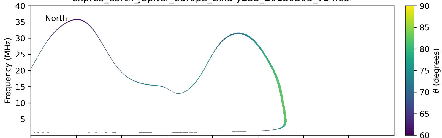
expres_earth_jupiter_europa_txka-y235_20180303_v14.cdf
