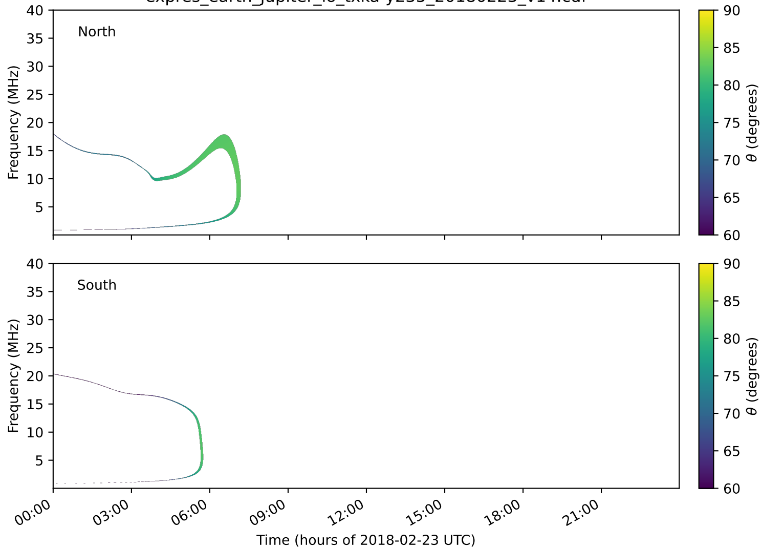
expres_earth_jupiter_io_txka-y235_20180223_v14.cdf
