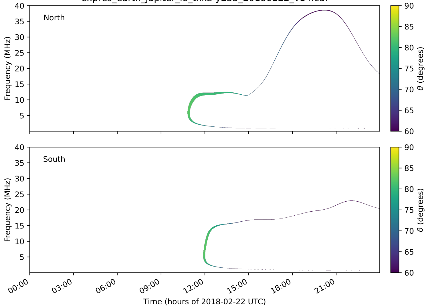
expres_earth_jupiter_io_txka-y235_20180222_v14.cdf
