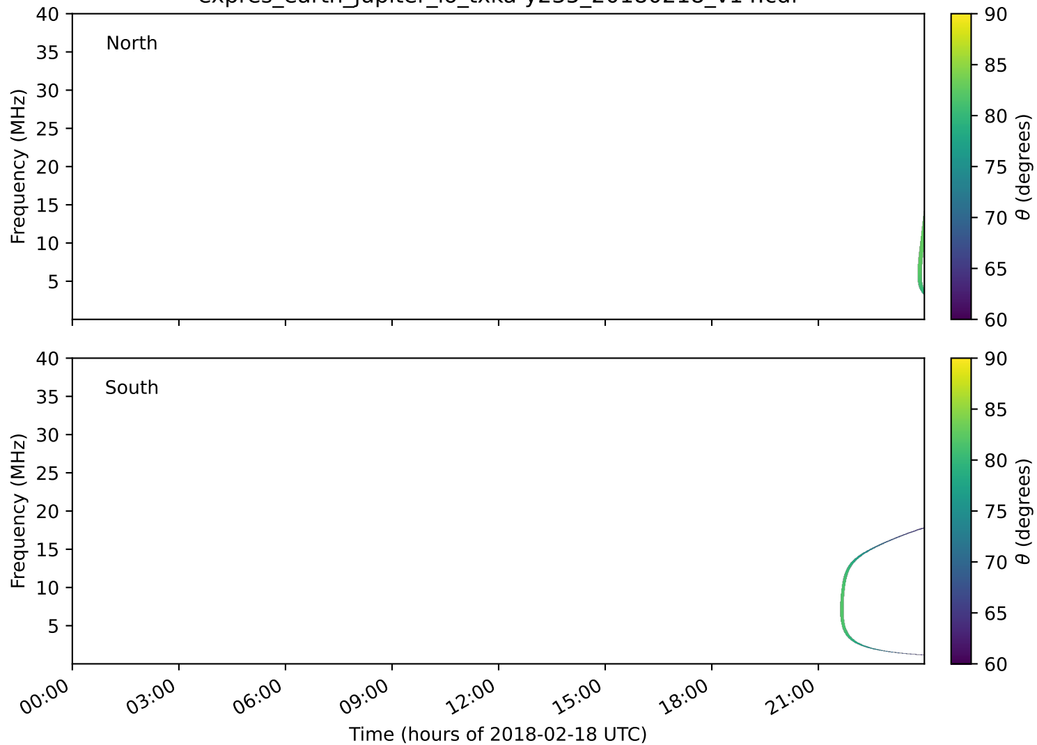
expres_earth_jupiter_io_txka-y235_20180218_v14.cdf
