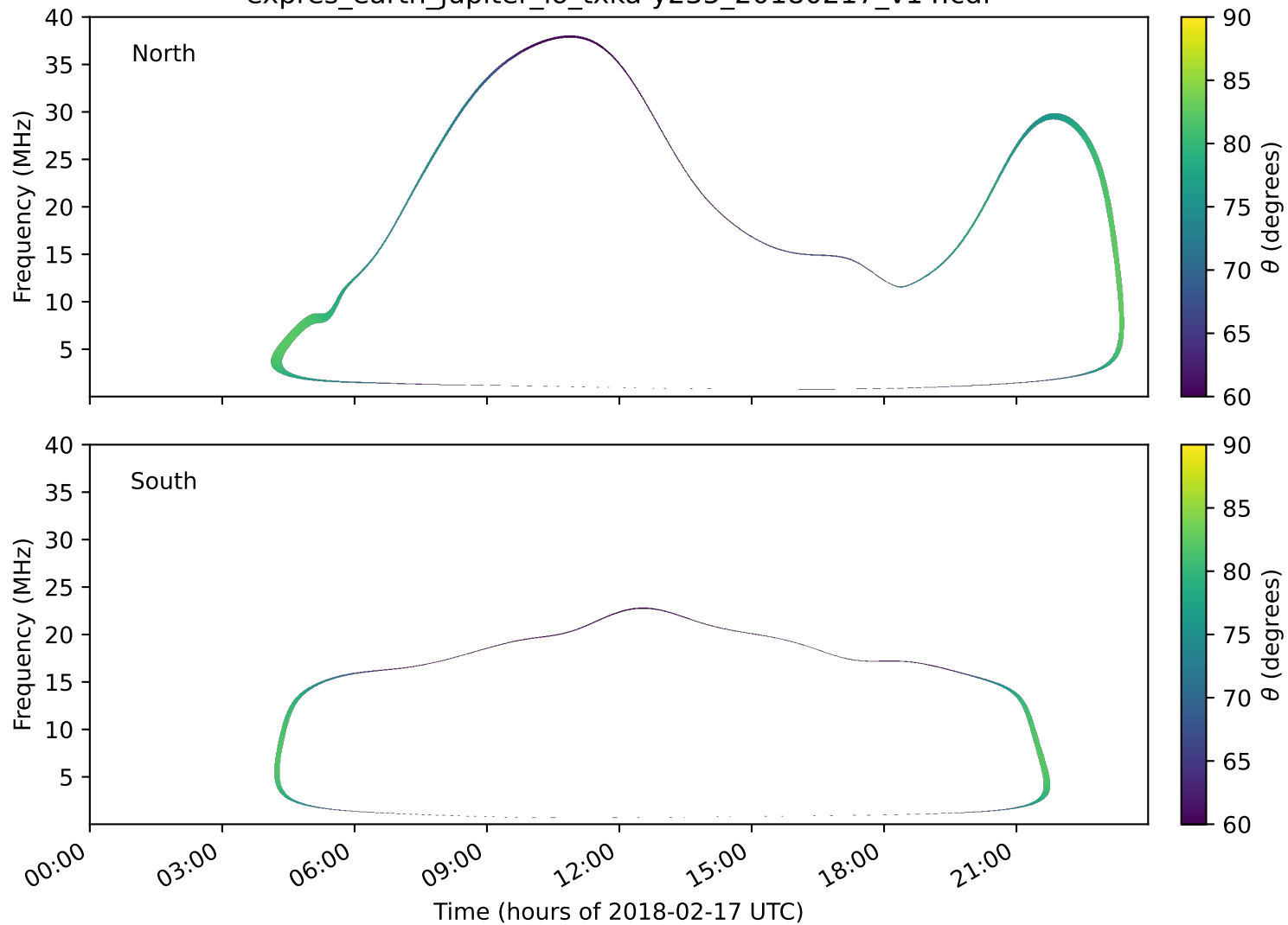
expres_earth_jupiter_io_txka-y235_20180217_v14.cdf
