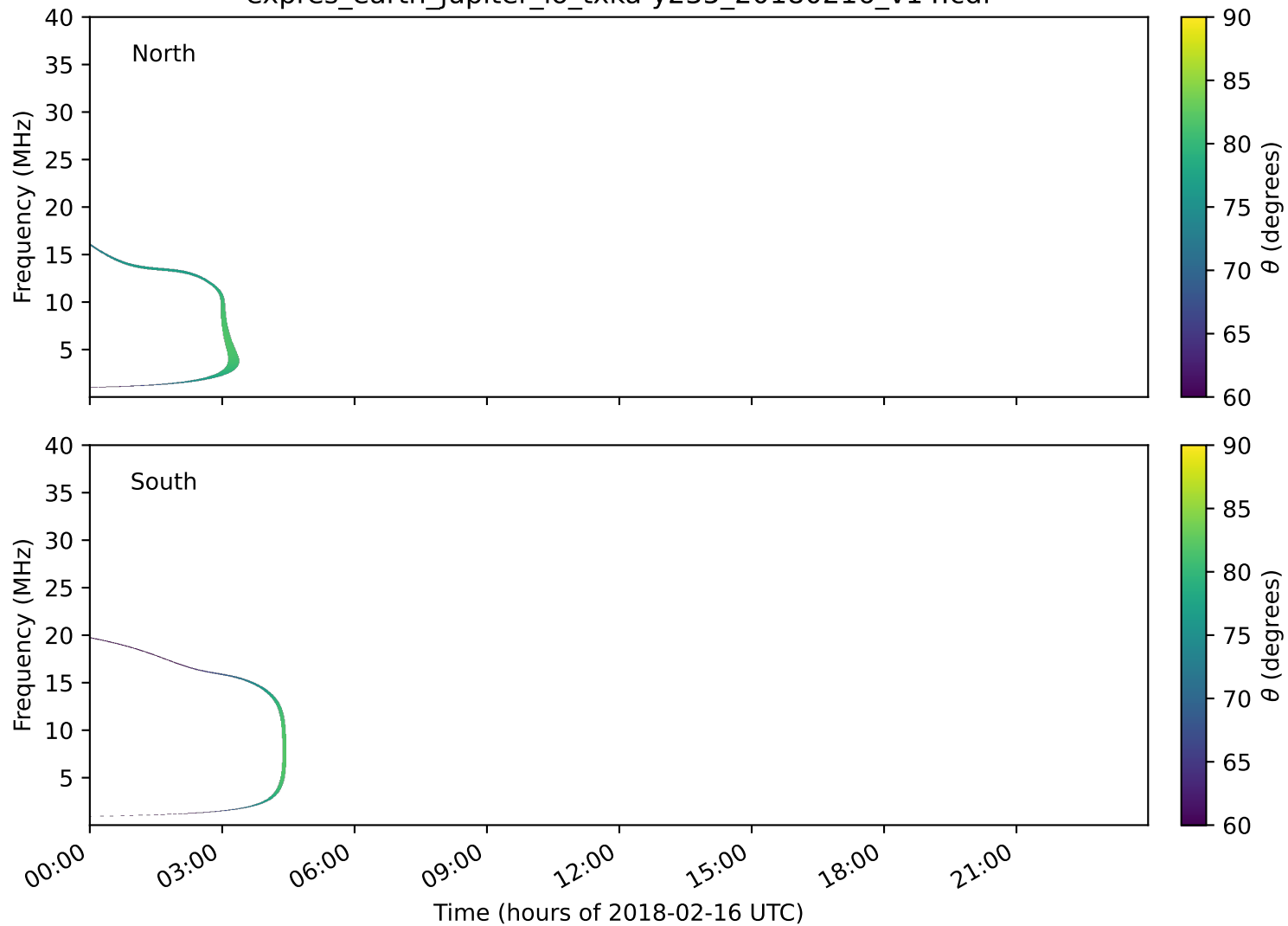
expres_earth_jupiter_io_txka-y235_20180216_v14.cdf
