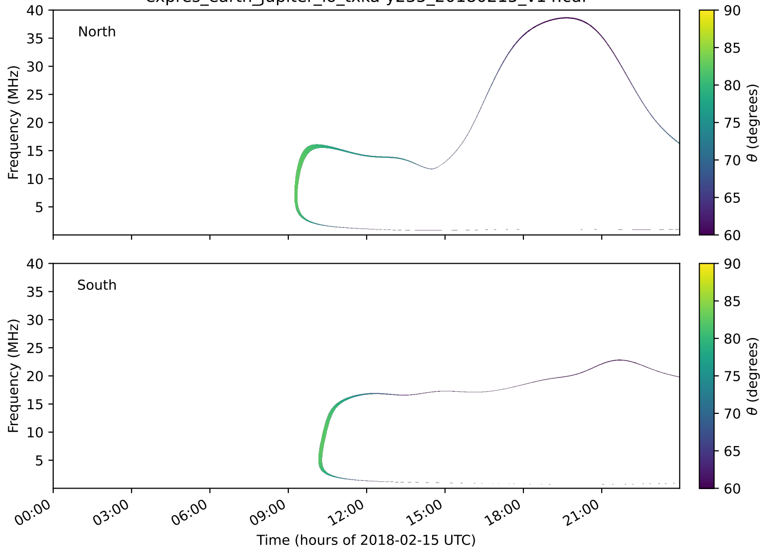
expres_earth_jupiter_io_txka-y235_20180215_v14.cdf
