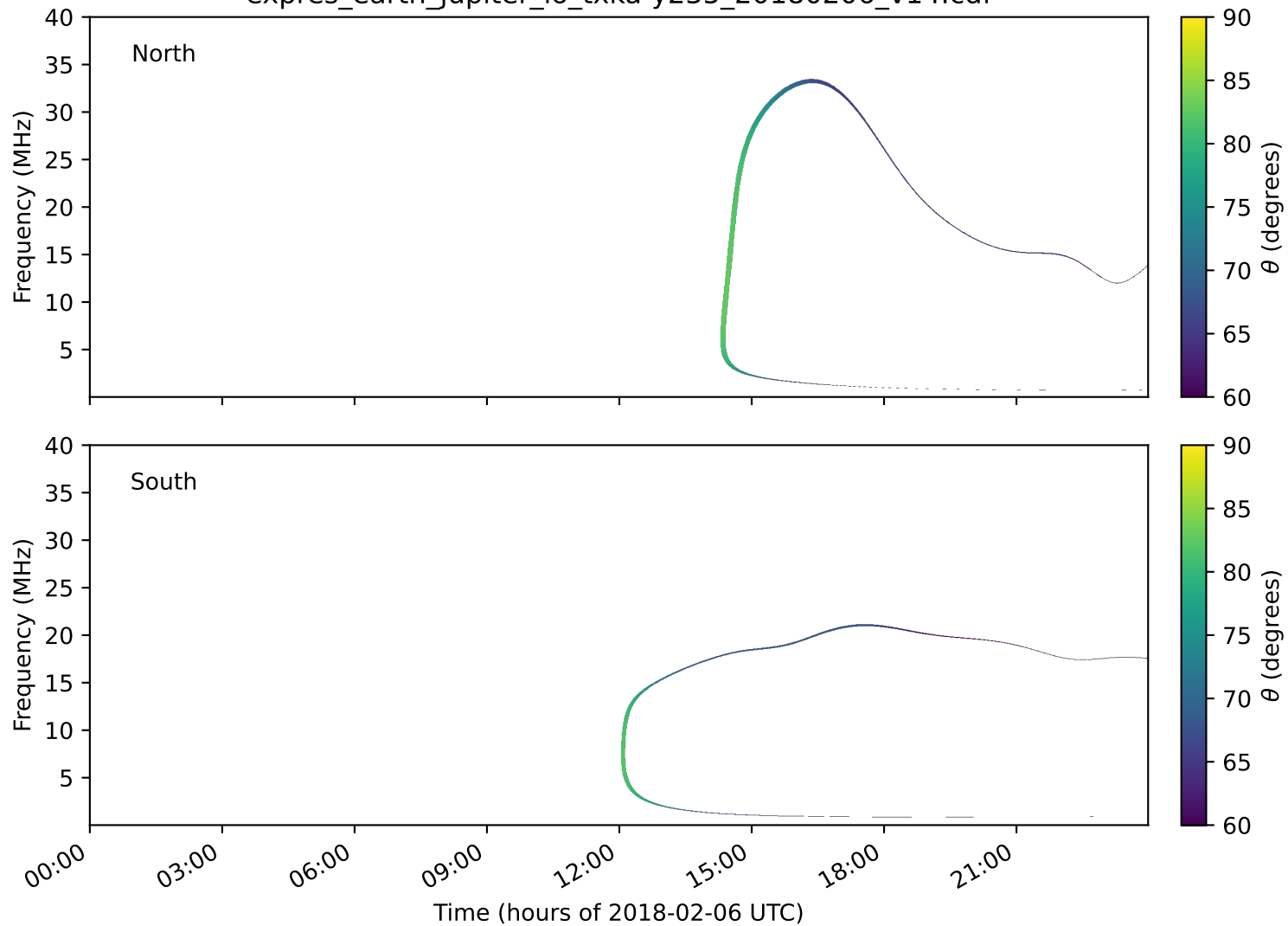
expres_earth_jupiter_io_txka-y235_20180206_v14.cdf
