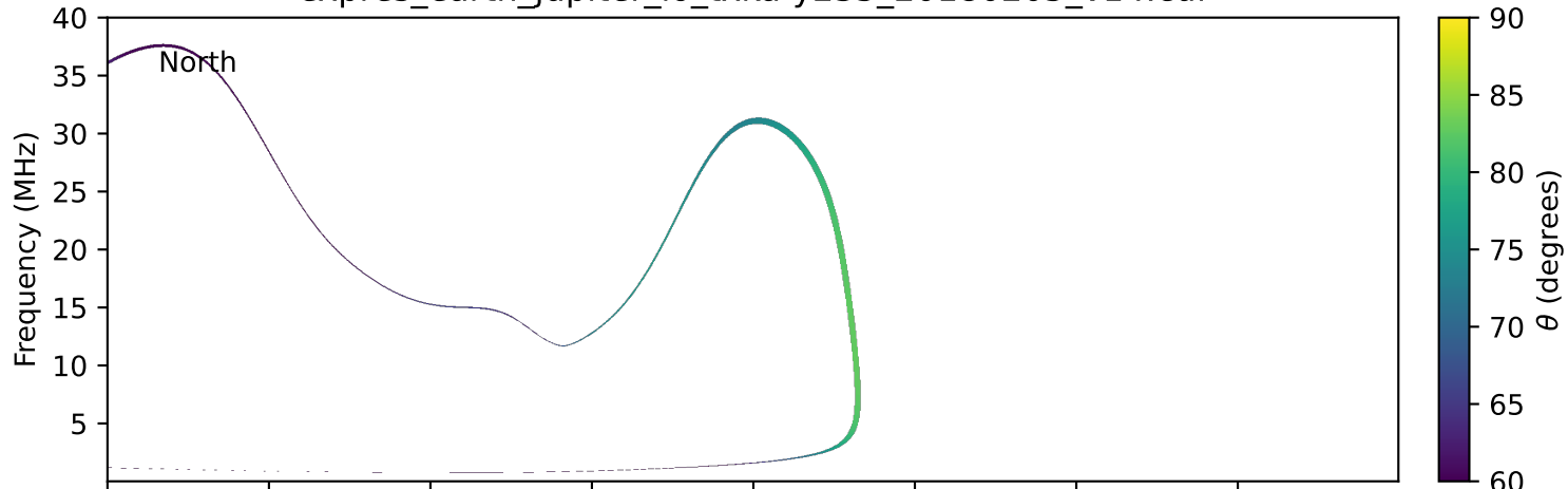
expres_earth_jupiter_io_txka-y235_20180205_v14.cdf
