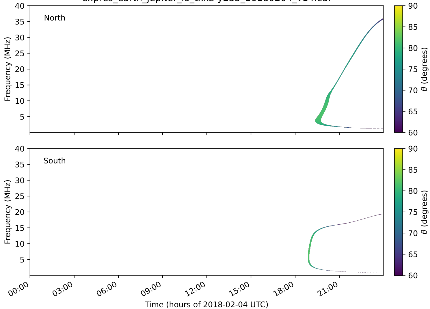
expres_earth_jupiter_io_txka-y235_20180204_v14.cdf
