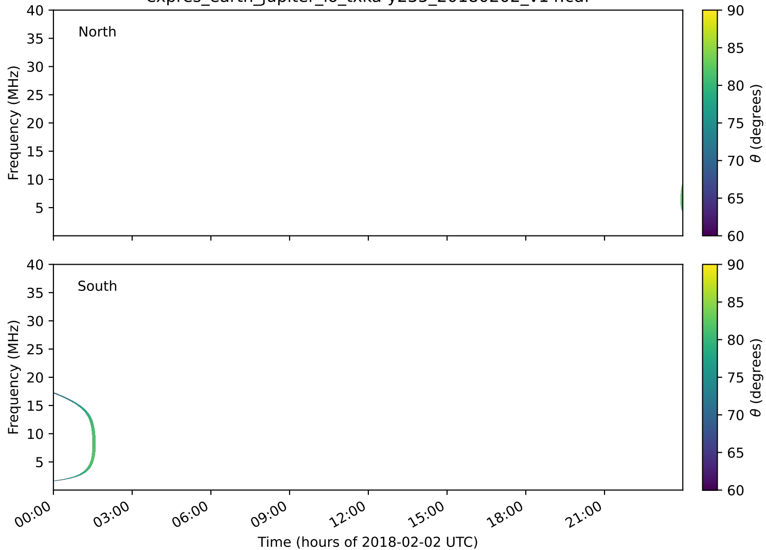
expres_earth_jupiter_io_txka-y235_20180202_v14.cdf
