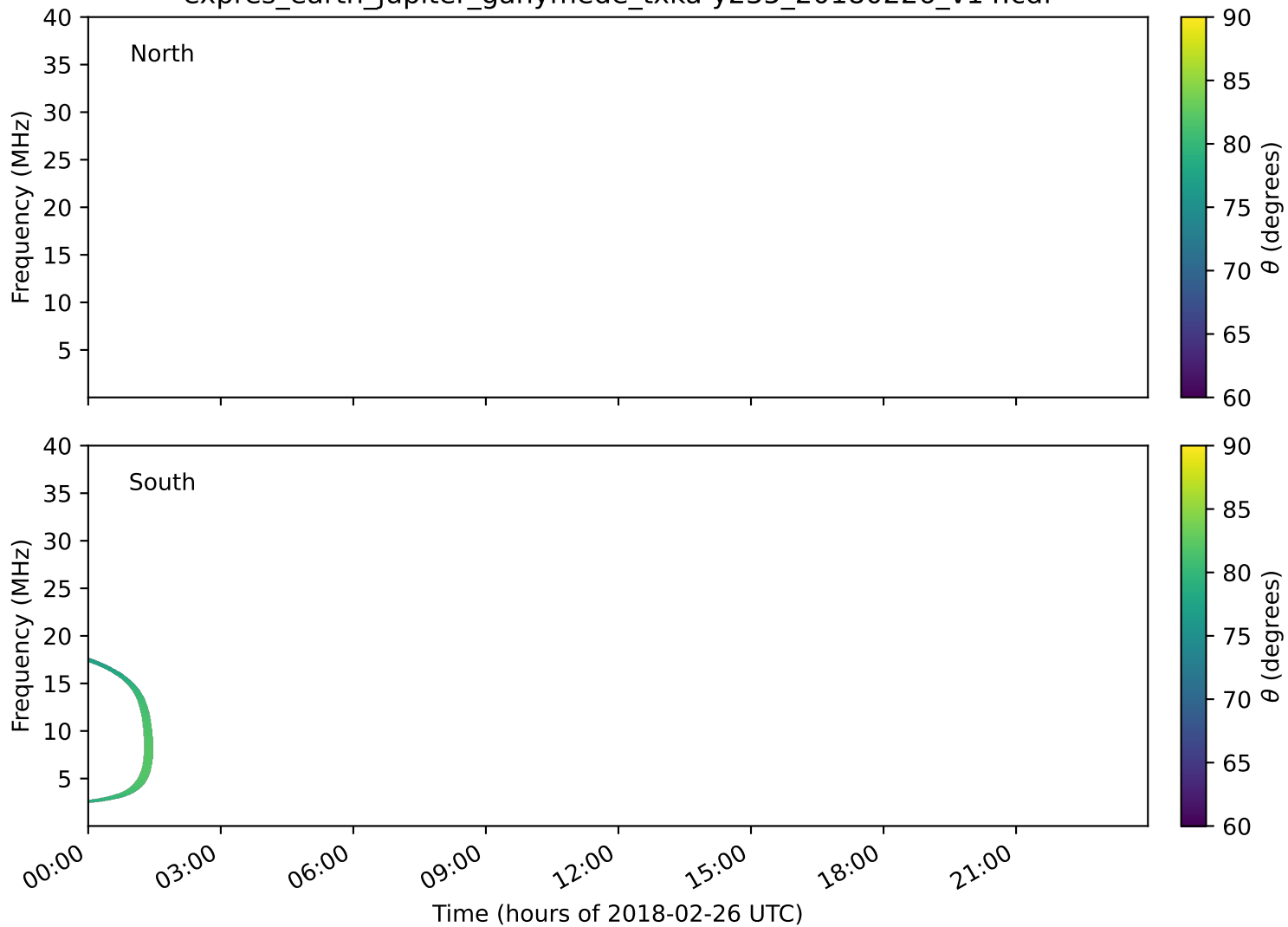
expres_earth_jupiter_ganymede_txka-y235_20180226_v14.cdf
