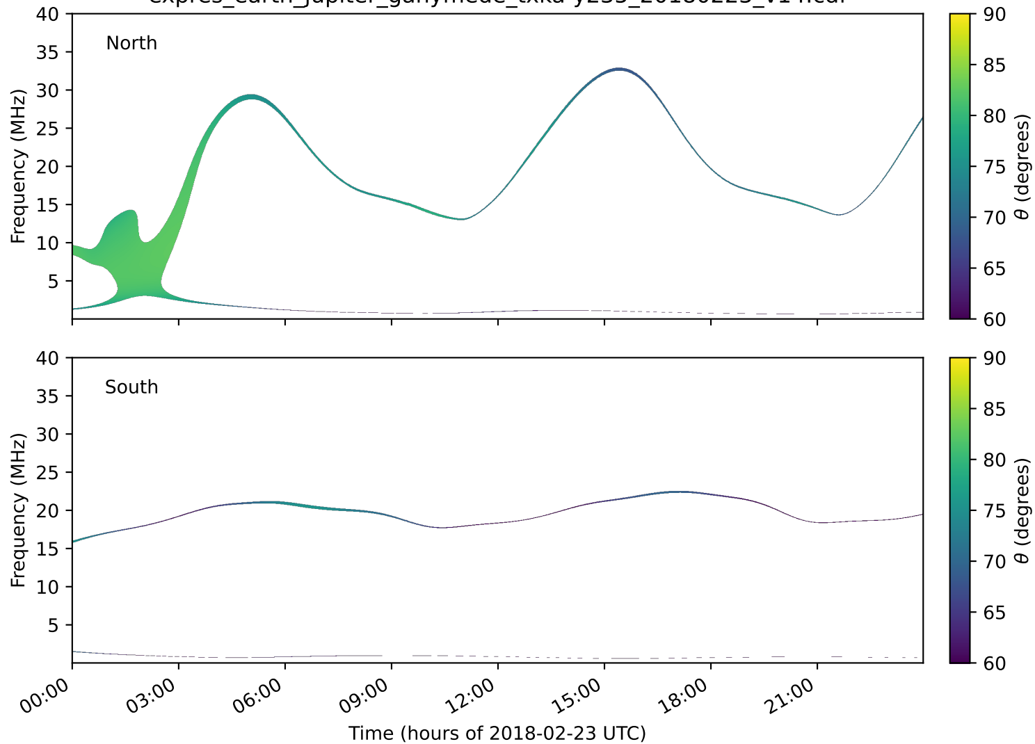
expres_earth_jupiter_ganymede_txka-y235_20180223_v14.cdf
