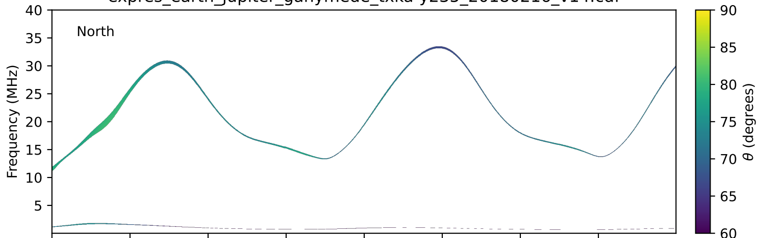
expres_earth_jupiter_ganymede_txka-y235_20180216_v14.cdf
