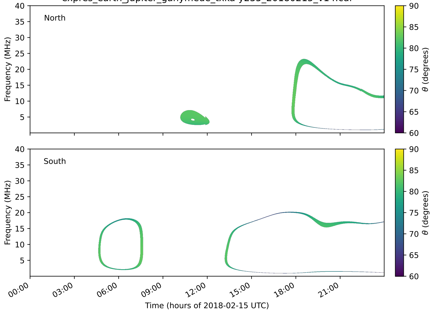
expres_earth_jupiter_ganymede_txka-y235_20180215_v14.cdf
