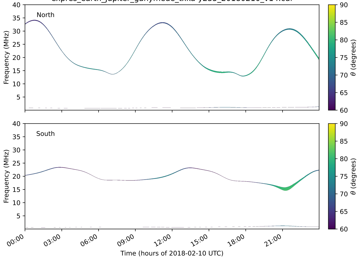
expres_earth_jupiter_ganymede_txka-y235_20180210_v14.cdf
