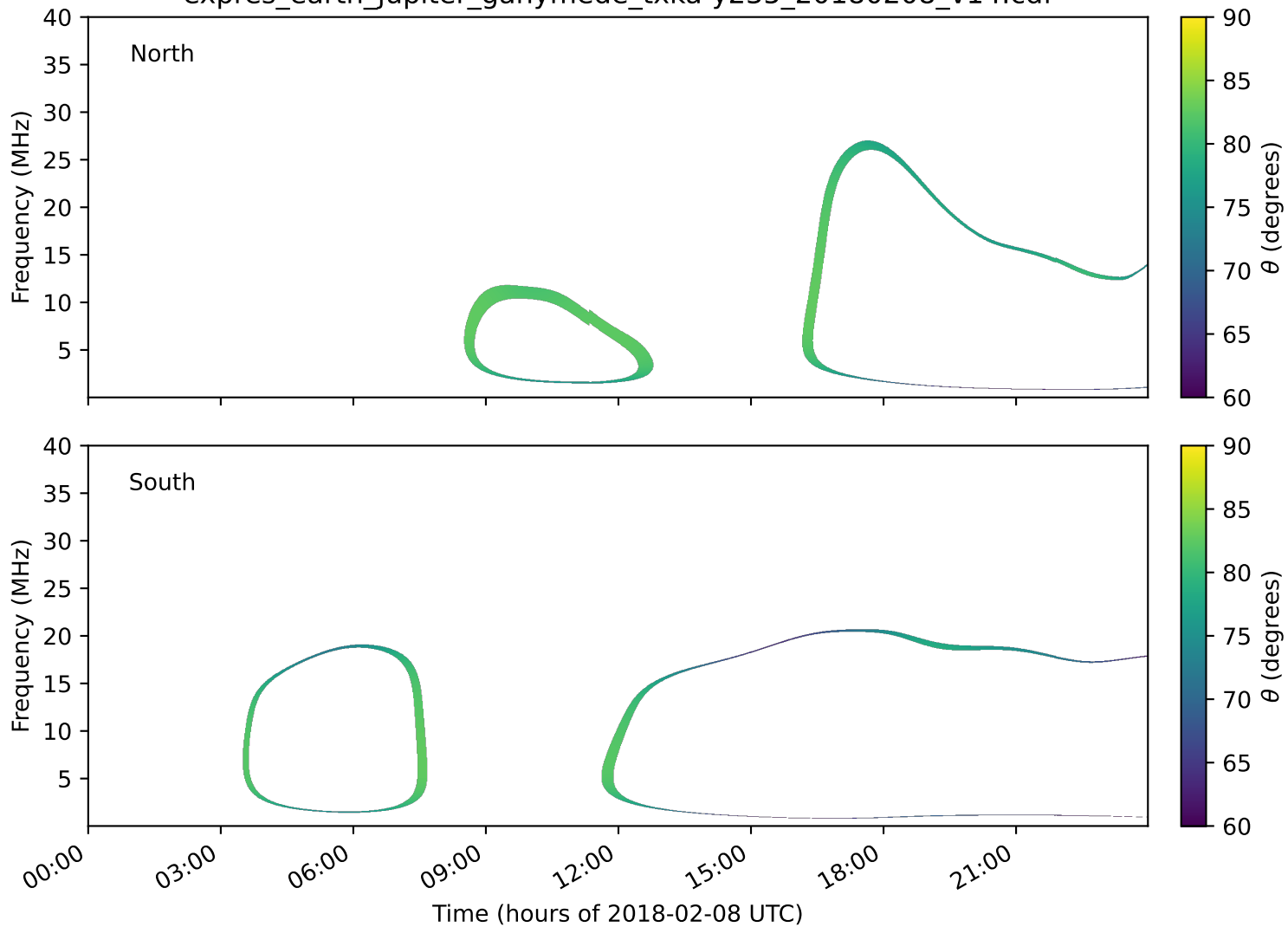
expres_earth_jupiter_ganymede_txka-y235_20180208_v14.cdf
