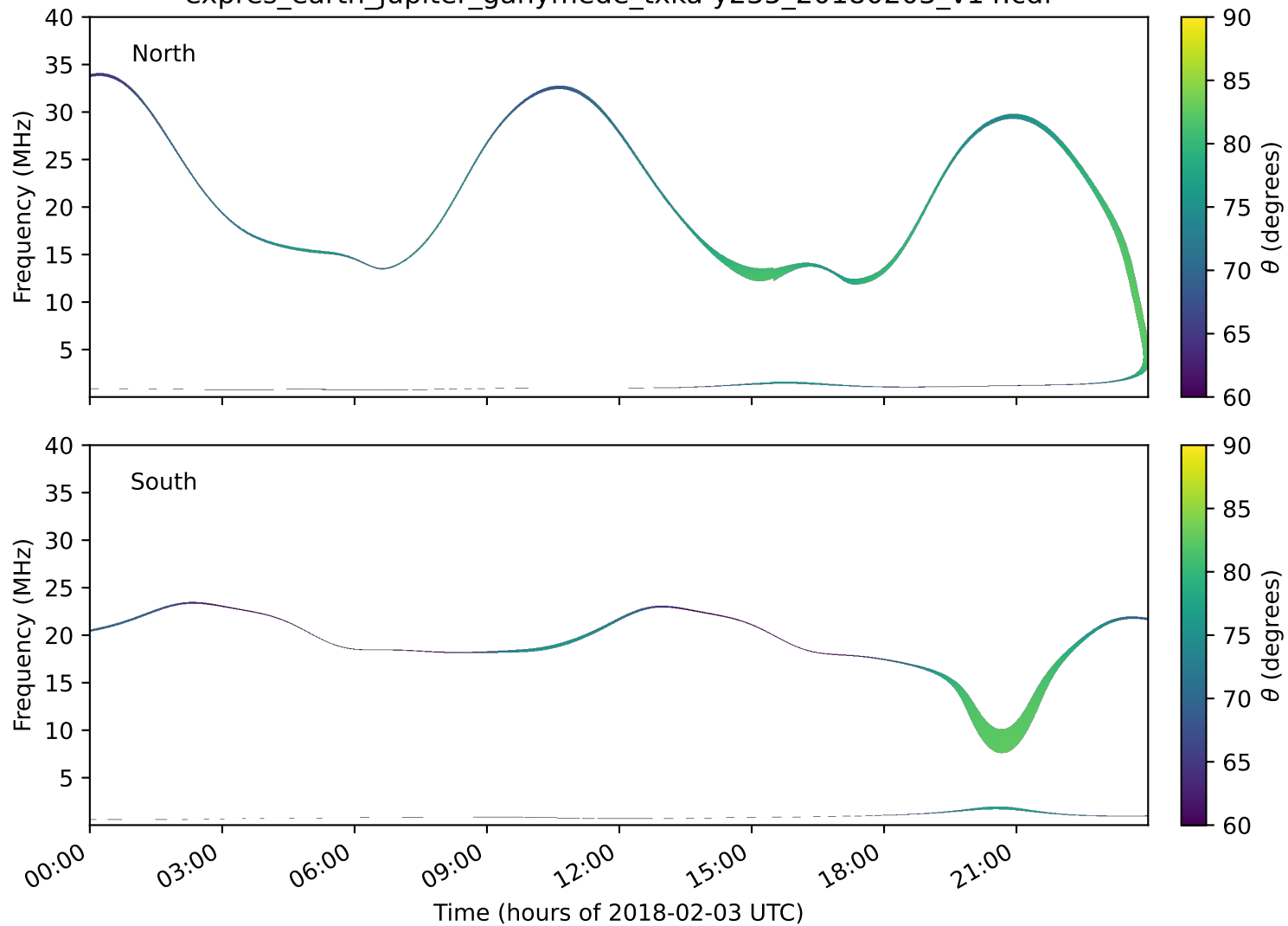
expres_earth_jupiter_ganymede_txka-y235_20180203_v14.cdf
